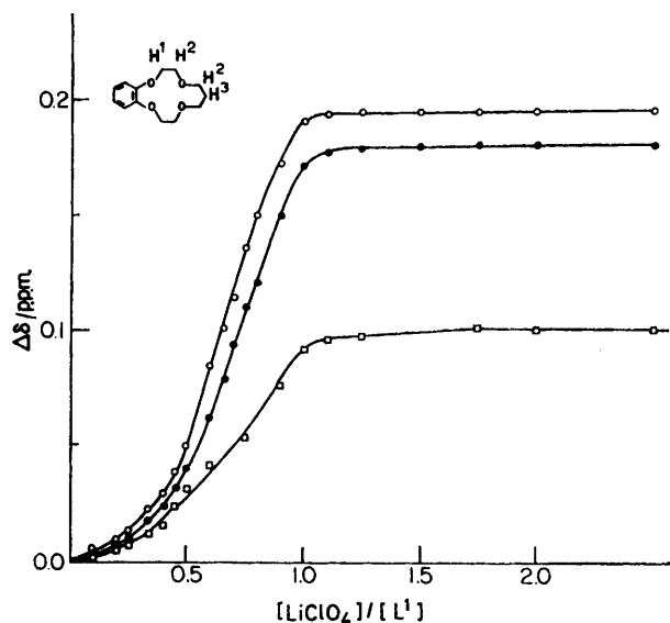
FIGURE 3 Increments of chemical shifts of proton signals of L 1 in nitromethane against [LiClO 4 ]:[L 1 ] ([L 1 ] = 10 -2 mol dm -3 ). H 1 (○), H 2 (●), and H 3 (□). Full lines correspond to the computed points
