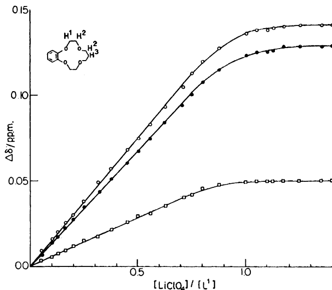
FIGURE 4 Increments of chemical shifts of proton signals of L 1 in acetonitrile against [LiClO 4 ]:[L 1 ] ([L 1 ] = 10 -2 mol dm -3 ). H 1 (○), H 2 (●), and H 3 (□). Full lines correspond to the computed points
