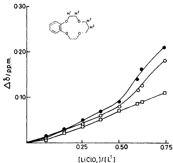
FIGURE 2 Increments of chemical shifts of proton signals of L 1 in methylene chloride against [LiClO 4 ]:[L 1 ] ([L 1 ] = 10 -3 mol dm -3 ). H 1 (●), H 2 (○), and H 3 (□). Full lines correspond to the computed points
