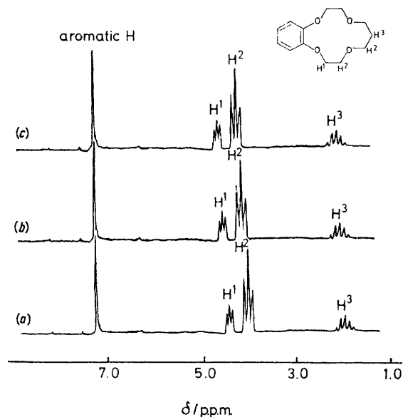
FIGURE 1 Hydrogen-1 n.m.r. spectra of 10 -2 mol dm -3 solutions of L 1 in nitromethane in the presence of Li[ClO 4 ]. Free ligand (a), [LiClO 4 ] : [L 1 ] = 1 : 2 (b), and [LiClO 4 ] : [L 1 ] = 1 : 1 (c)
